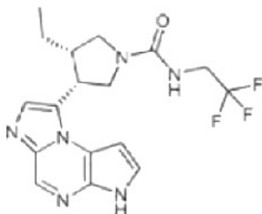
Chemical structure of upadacitinib
